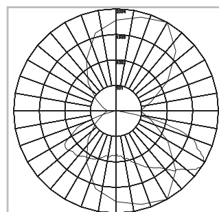
LIGHT DISTRIBUTION CURVE (LDC) 1476-3K-60W
